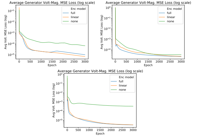
Fig. 5. Average MSE error (log scale) during training phase for generator voltage magnitude predictions. Top-left: 39_epri, Top-right: 189_edin, bottom: 2848_rte
